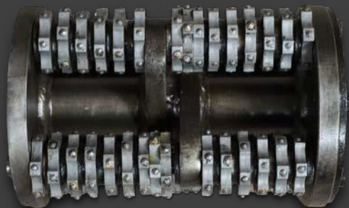
M200HD4 - $633.00 8" carbide flail cutters cage assembly including drum and 60 x TCT cutters. Replacement cutters available (sold separately).
